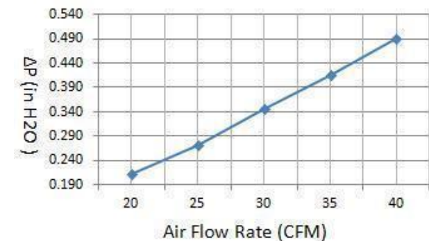
ΔP VS Air Flow Rate Chart
