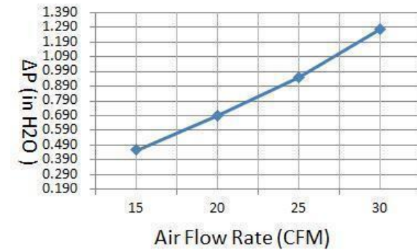
ΔP VS Air Flow Rate Chart
