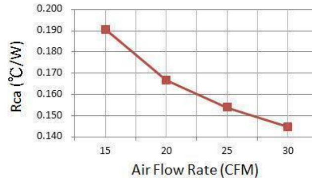
Rca VS Air Flow Rate Chart
