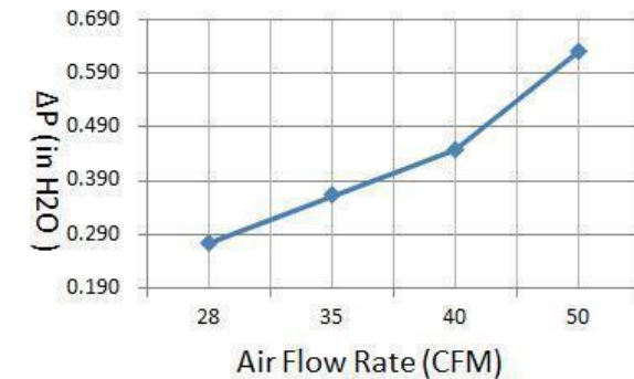
ΔP VS Air Flow Rate Chart
